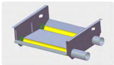
Stainless Steel Sheet used for Long Life of Auger Casing
