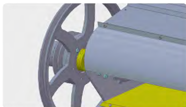
Safety Clutch Provision for Feeder
